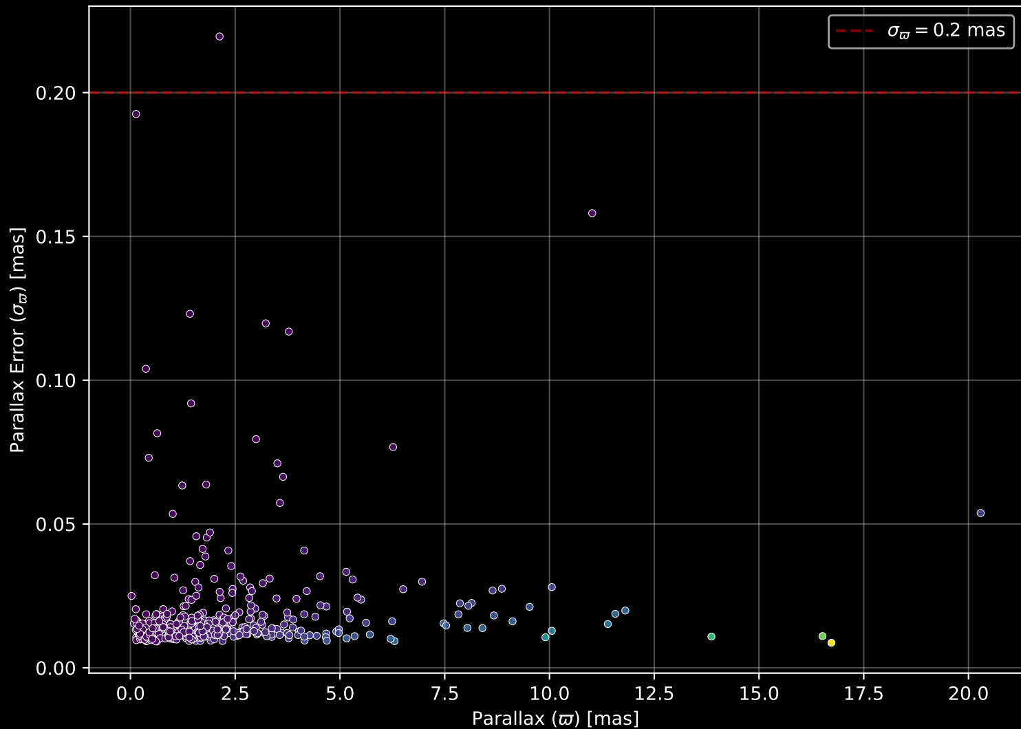
APOGEE DR17 Field: [120+30] Parallax Quality (n= 393)
