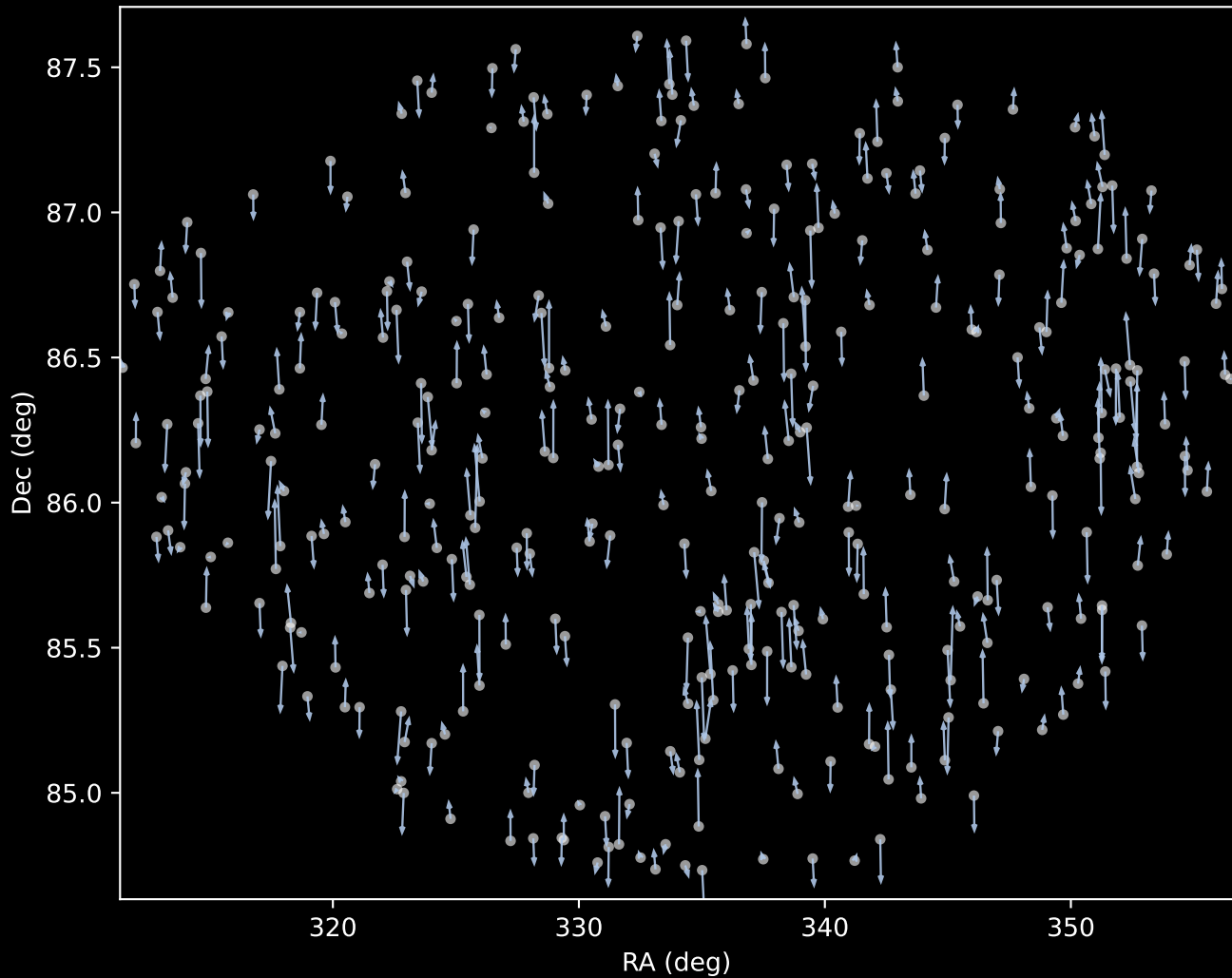
APOGEE DR17 Cluster 1 Proper Motion Vectors (n=347)
