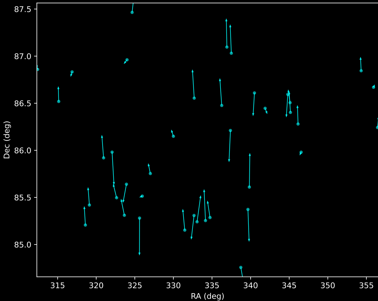
APOGEE DR17 Noise Stream Proper Motion Vectors (n=39)
