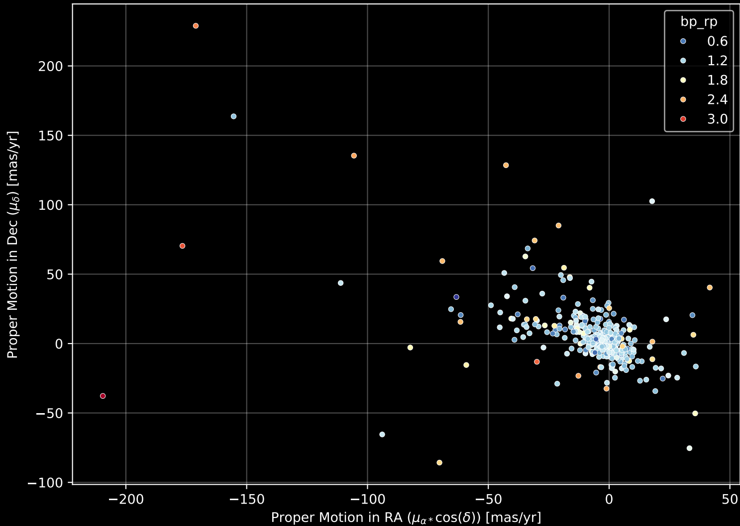
APOGEE DR17 Field: [120+30] Proper Motion Diagram (n= 393)
