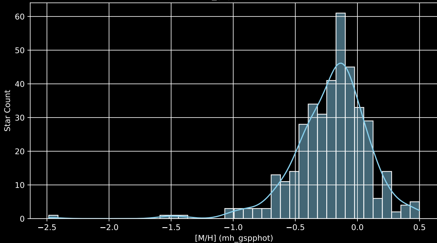
APOGEE DR17 Field: [120+30 [M/H] (mh_gspphot) (n= 390)
