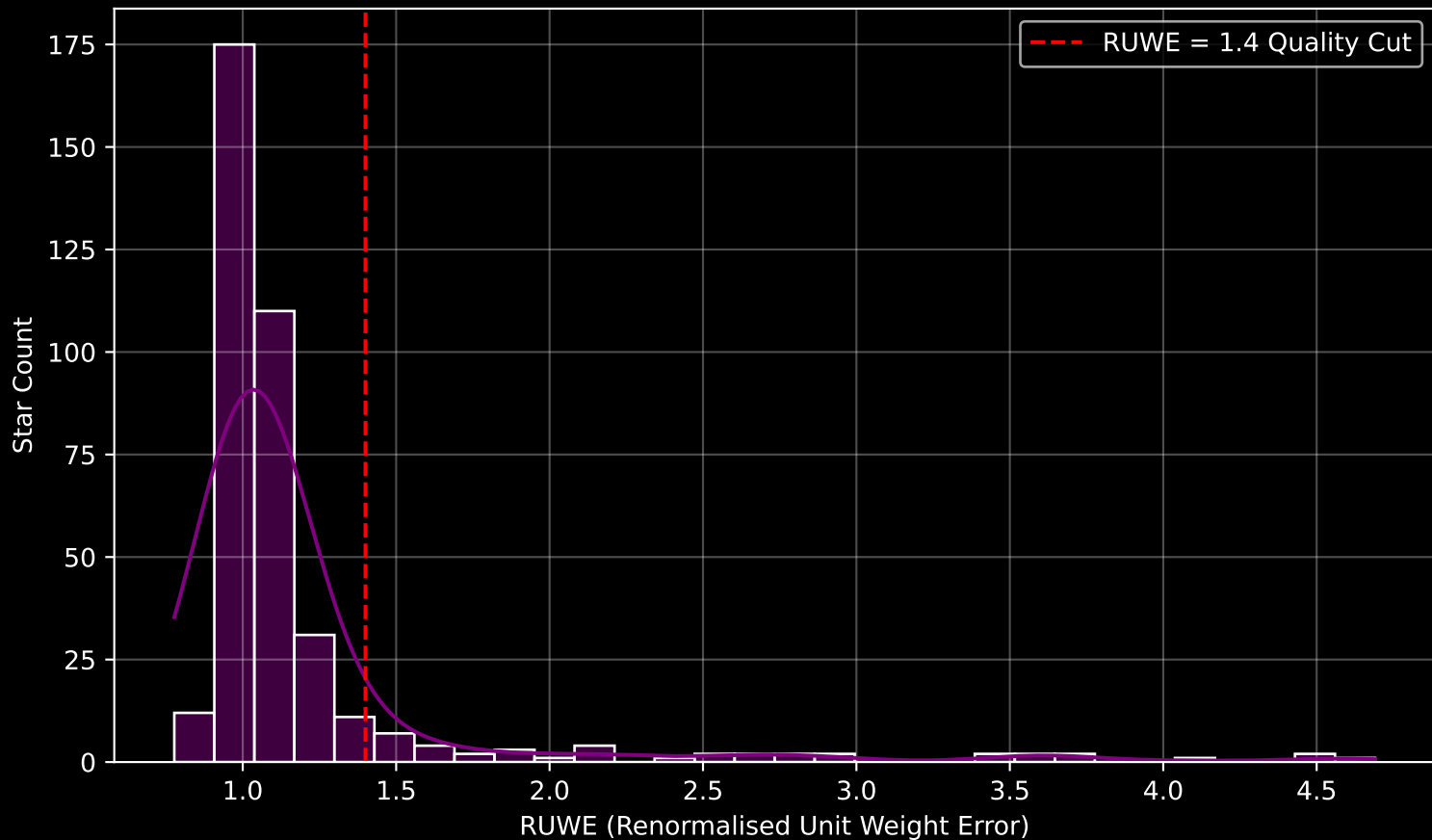
GAPOGEE DR17 Field [120+30] RUWE Distribution (n= 379)
